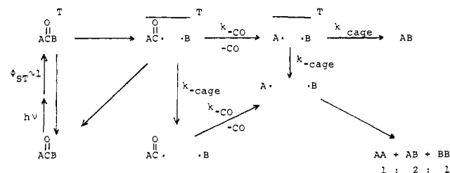
Scheme I. Possible Routes to Diarylethanes (AA, 2; AB, 3; BB, 4) from 1,3-Diarylpropan-2-one (AC(=O)B) Photodecarbonylations
