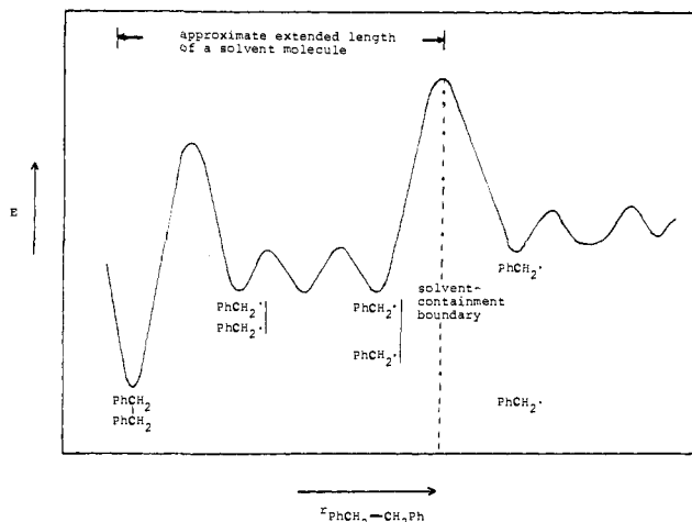
Figure 1. Representation of energy vs. separation of benzyl radical pairs in a smectic phase.
