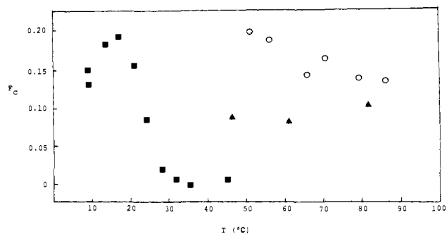
Figure 2. Fraction of in-cage benzyl radical recombination ( F_c ) from photolysis of 1a in BS (■), BCCN (▲), and CCl 4 /CN (○) vs. temperature.
